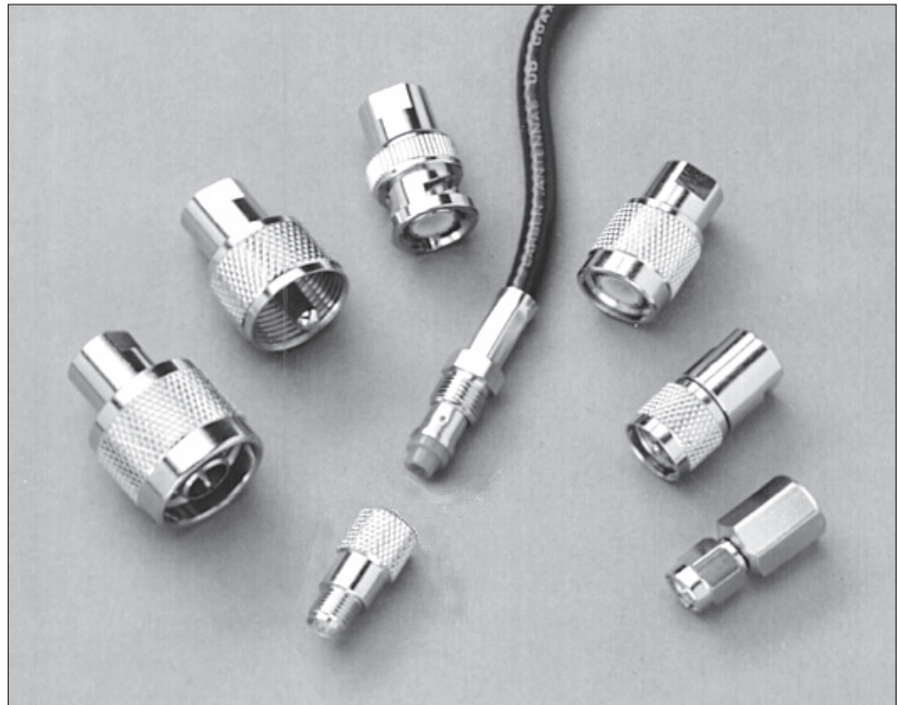
Left to right: N, PL, BNC, TNC, Mini-UHF, SMA male. Center: SMA Female
